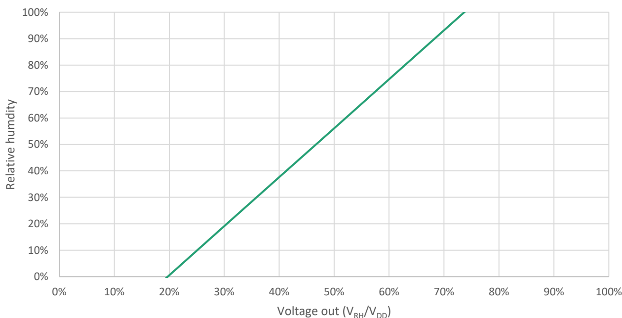
Figure 2: Relationship between the ratiometric analog voltage output and the measured relative humidity
