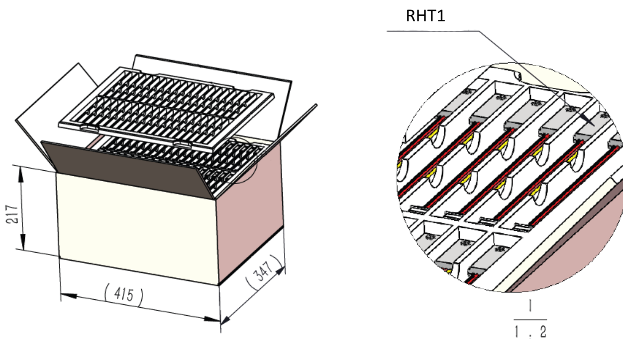
Figure 6: Packaging details
