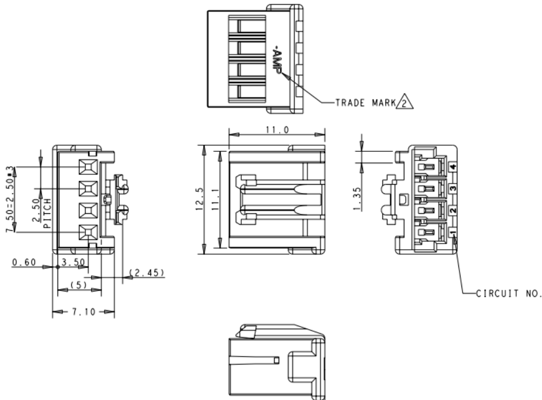
Figure 4: TE-917688 connector drawing 2
