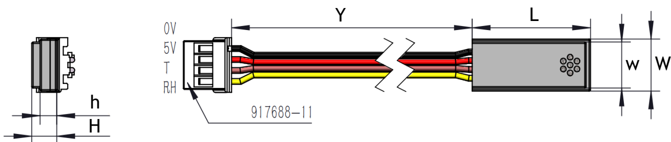
Figure 3: Outline dimensions RHT1
