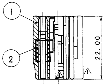
SEC. B-B
