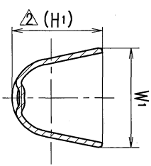
SEC. C-C
