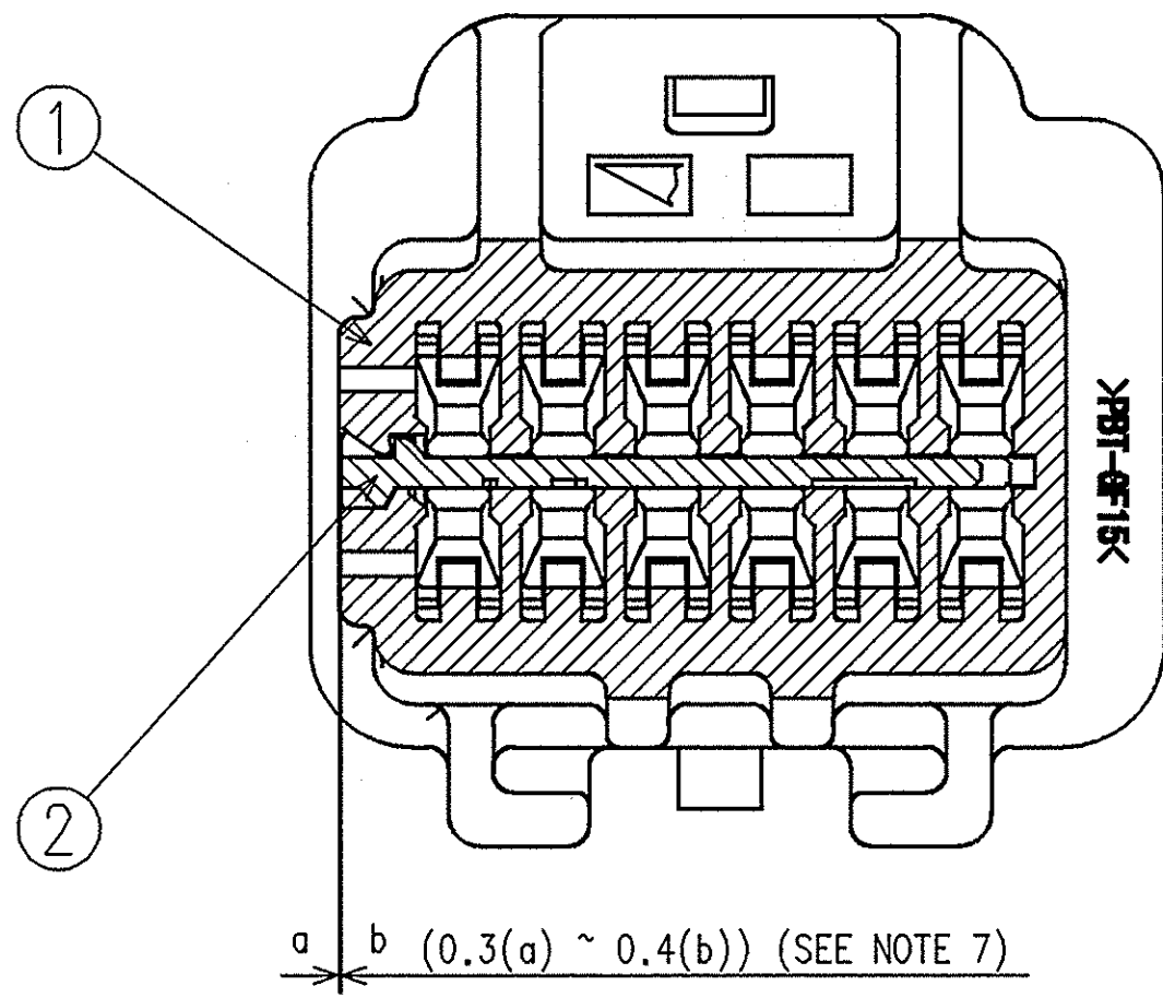
SECTION B-B
