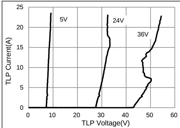
Fig.4 TLP Measurement
