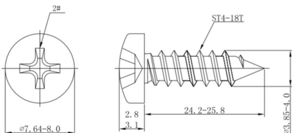
Screw 4PCS
