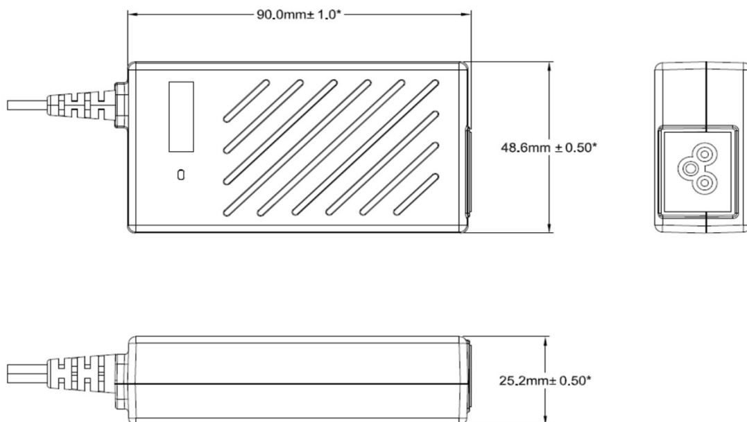
FWA020-Class I-DWG
