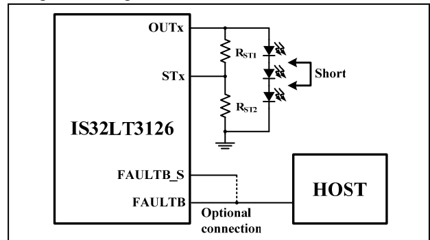
Figure 3 STx Pins Operation
