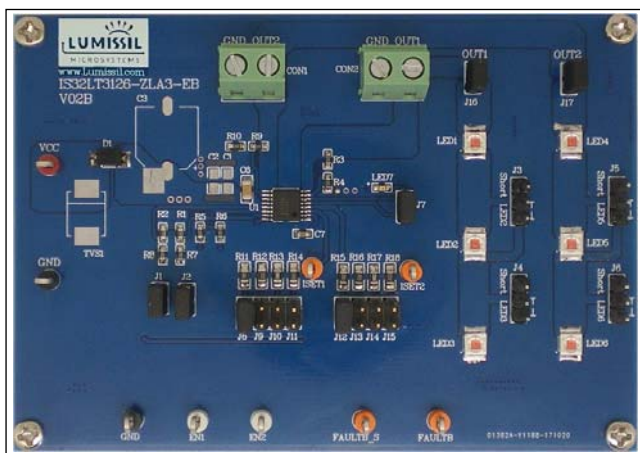
Figure 1 Photo of IS32LT3126 Evaluation Board
