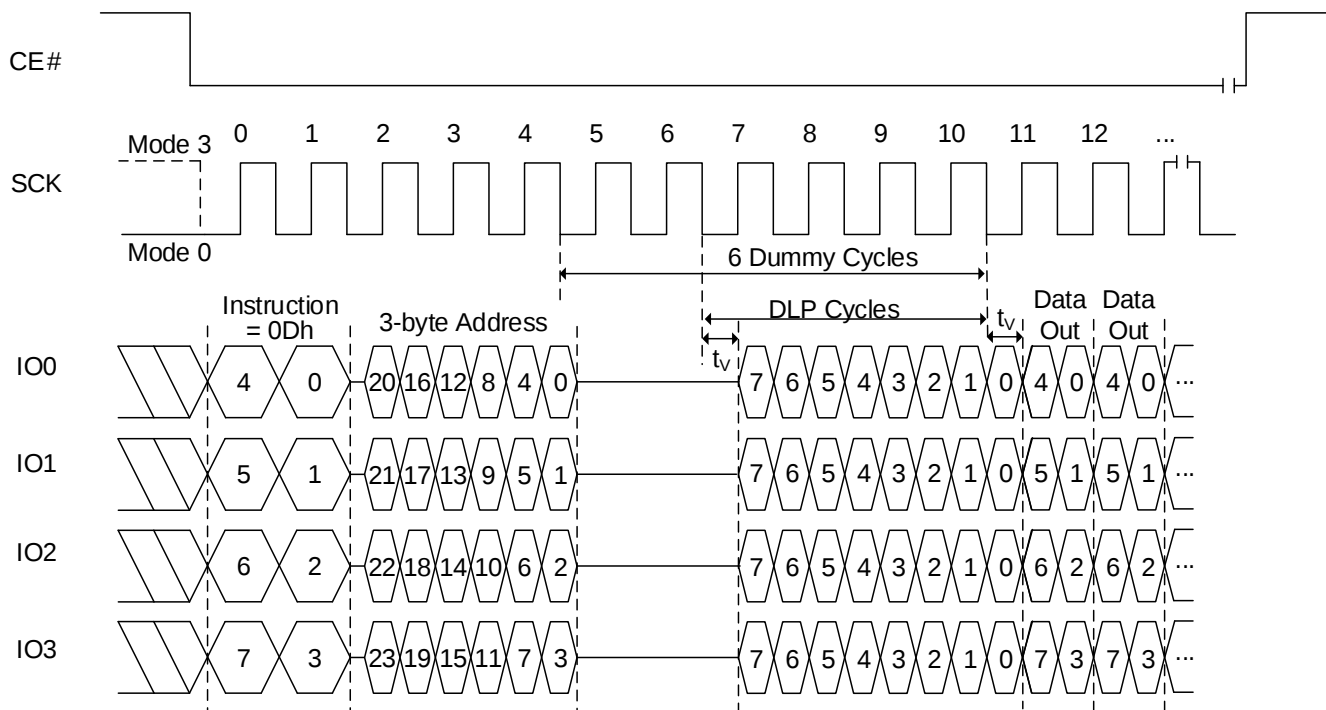
Figure 8.147 FRDTR Sequence with DLP In QPI Mode (0Dh [EXTADD=0], 3-byte address)
