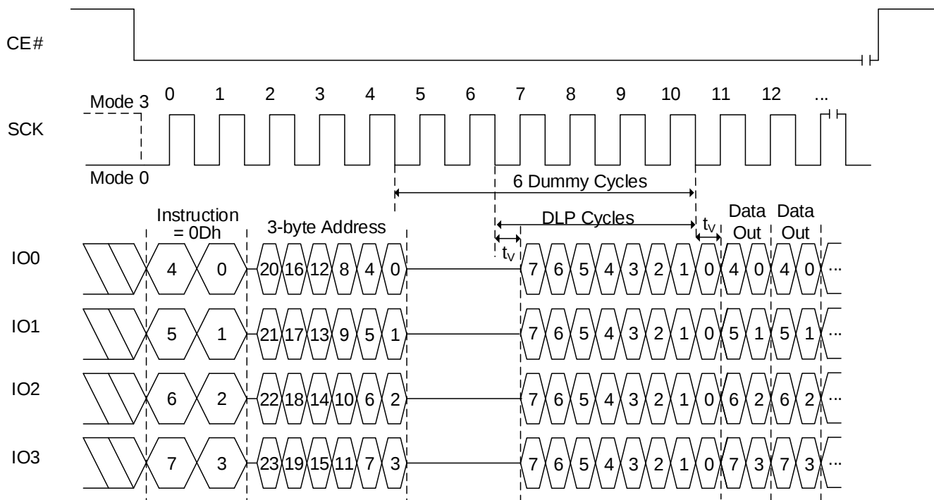
Figure 8.143 FRDTR Sequence with DLP In QPI Mode (0Dh [EXTADD=0], 3-byte address)
