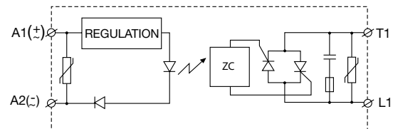
AC control
