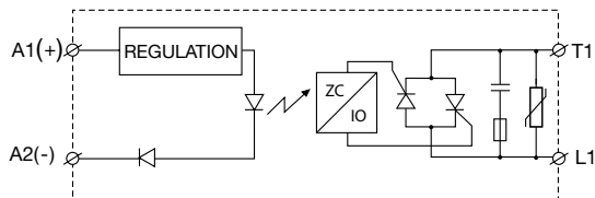
DC control
