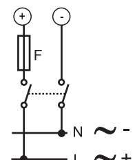
Fig. 17 Auxiliary power supply (H). 250 V [T] 630 mA fuse (F). Auxiliary power supply (L). 250 V [T] 3.15 A fuse (F).
