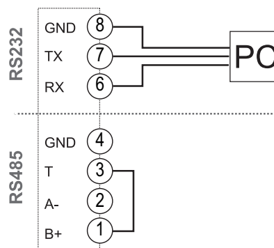
Fig. 26 M C 485232. RS232 serial port.
