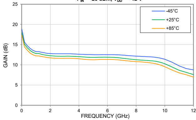
GAIN vs. TEMPERATURE, P_{IN} = -25 dBm, V_{DD} = +12 V
