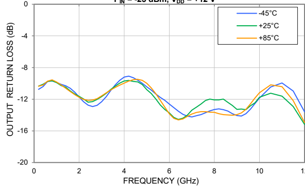
OUTPUT RETURN LOSS vs. TEMPERATURE, P_{IN} = -25 dBm, V_{DD} = +12 V
