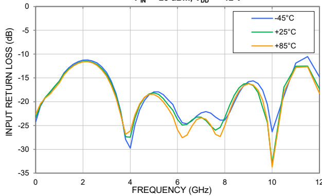
INPUT RETURN LOSS vs. TEMPERATURE, P_{IN} = -25 dBm, V_{DD} = +12 V
