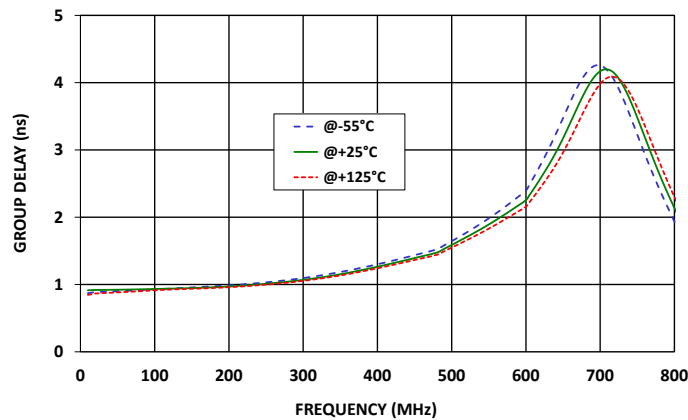
LFCG-510+ GROUP DELAY
