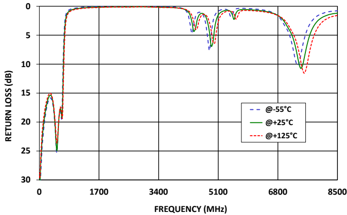
LFCG-510+ RETURN LOSS
