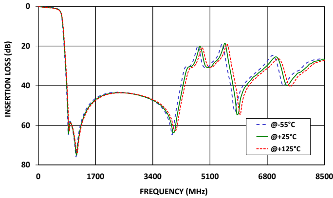
LFCG-510+ INSERTION LOSS
