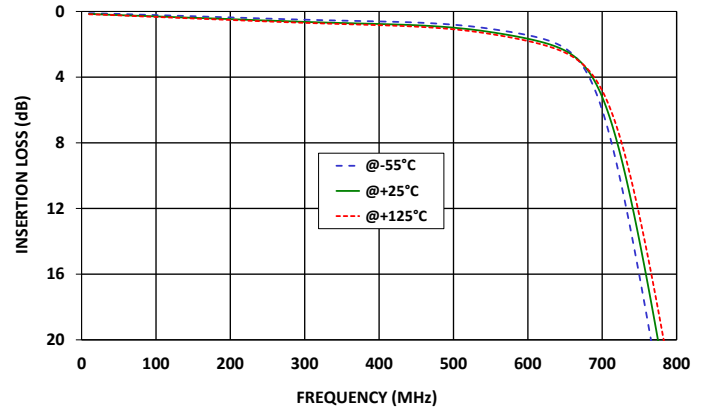
LFCG-510+ INSERTION LOSS (Zoomed)
