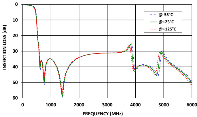
LFCG-320+ INSERTION LOSS
