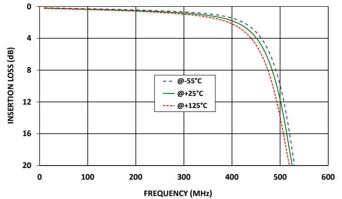
LFCG-320+ INSERTION LOSS (Zoomed)
