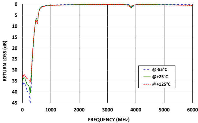
LFCG-320+ RETURN LOSS
