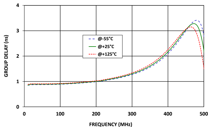
LFCG-320+ GROUP DELAY
