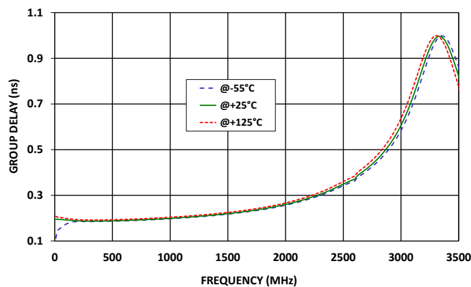
LFCG-2750+ GROUP DELAY
