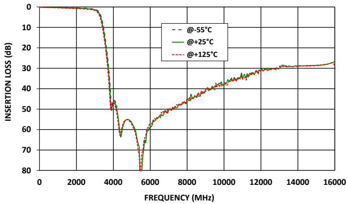
LFCG-2750+ INSERTION LOSS
