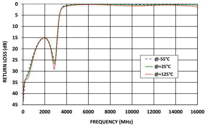
LFCG-2750+ RETURN LOSS
