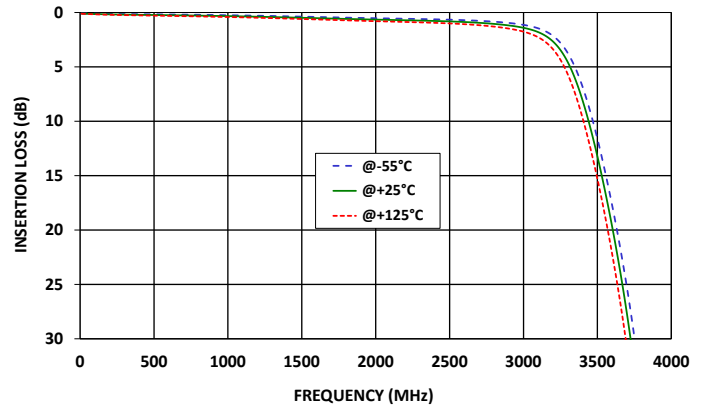
LFCG-2750+ INSERTION LOSS (Zoomed)
