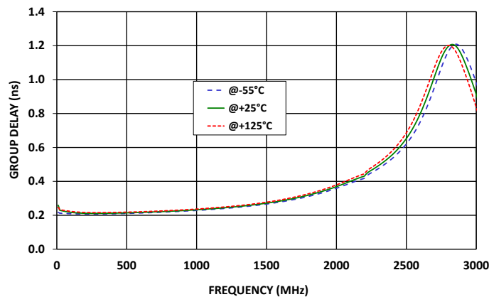
LFCG-2275+ GROUP DELAY
