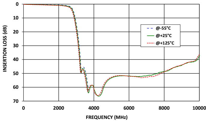
LFCG-2275+ INSERTION LOSS
