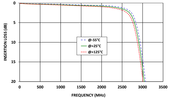
LFCG-2275+ INSERTION LOSS (Zoomed)
