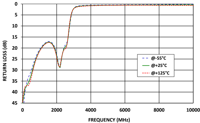
LFCG-2275+ RETURN LOSS
