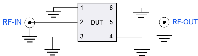
Fig 1. Block diagram of Test Circuit used for characterization, Test board TB-934-8C+ Conditions: Attenuation, VSWR: P_{IN} = 0 dBm
