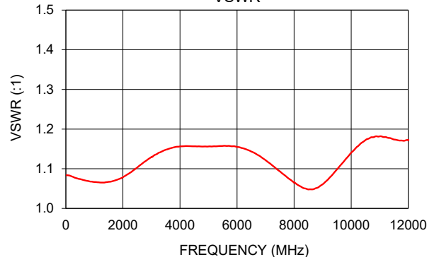
FW-1A+ VSWR
