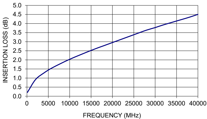
E40-3FT-KMKM+ INSERTION LOSS
