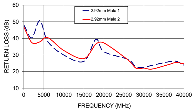
E40-3FT-KMKM+ RETURN LOSS
