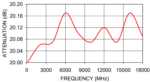
BW-S20W5+ ATTENUATION
