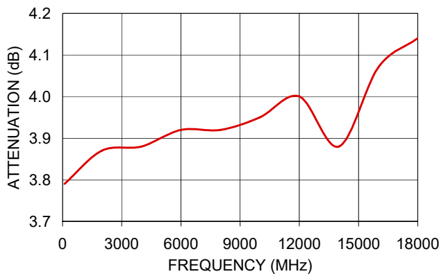
BW-N4W5+ ATTENUATION
