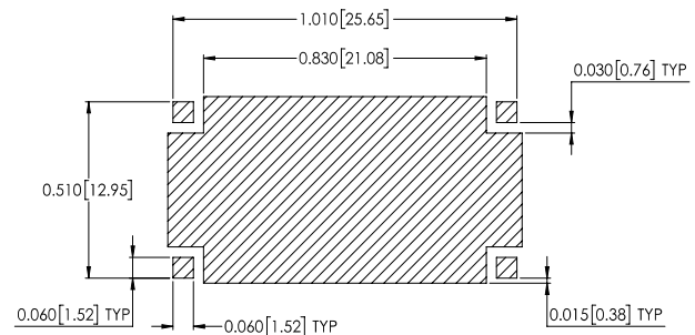
Suggested PCB Land Pattern
