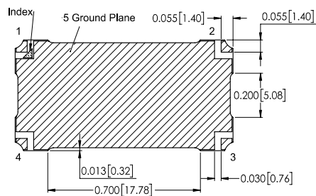
Suggested PCB Land Pattern
