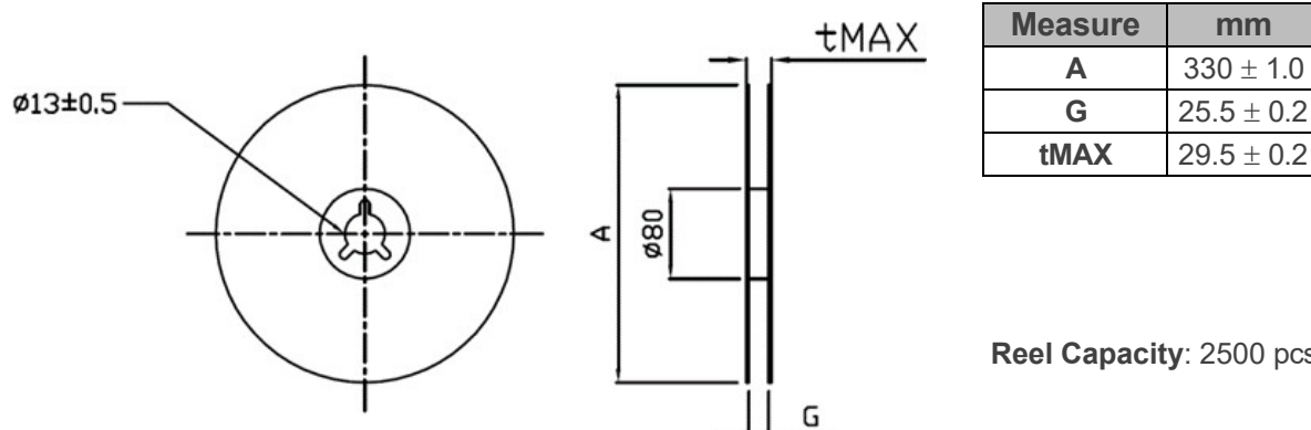
Figure 14 – Reel Dimensions and Capacity.
