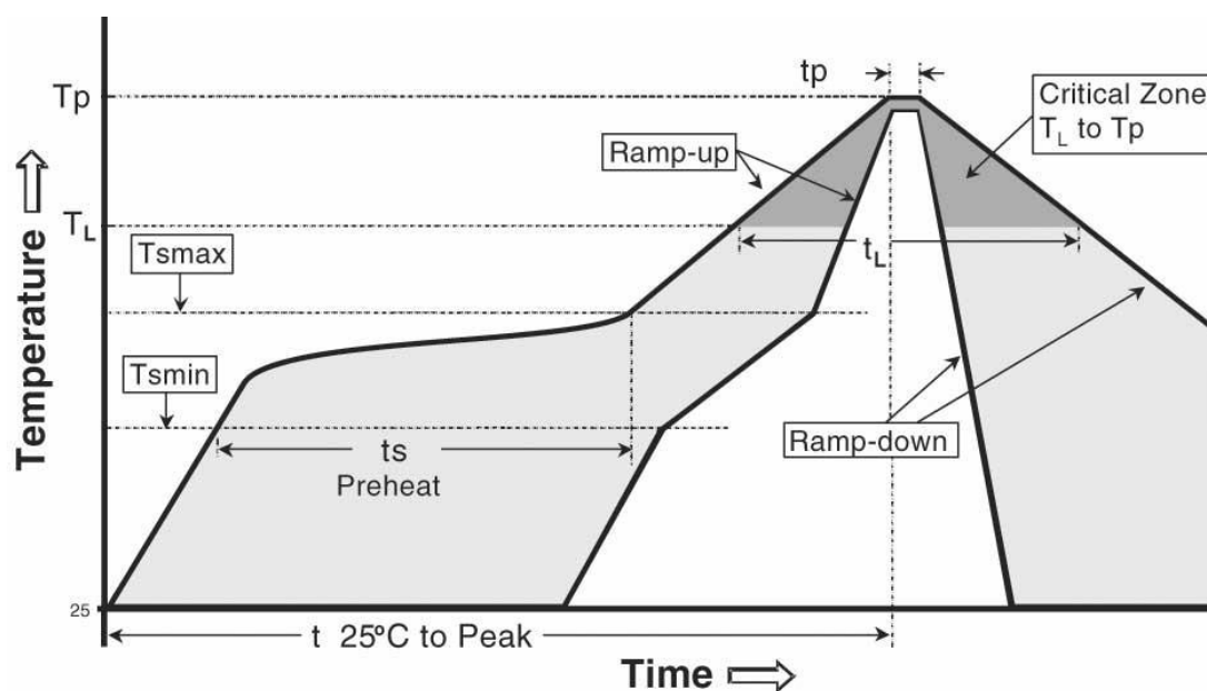
Figure 11 – Temperature profile.
