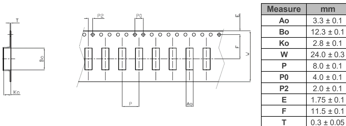
Figure 12 - Tape dimensions and tolerances.
