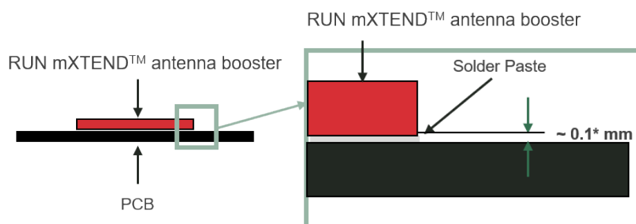
Figure 10 – Soldering Details.
