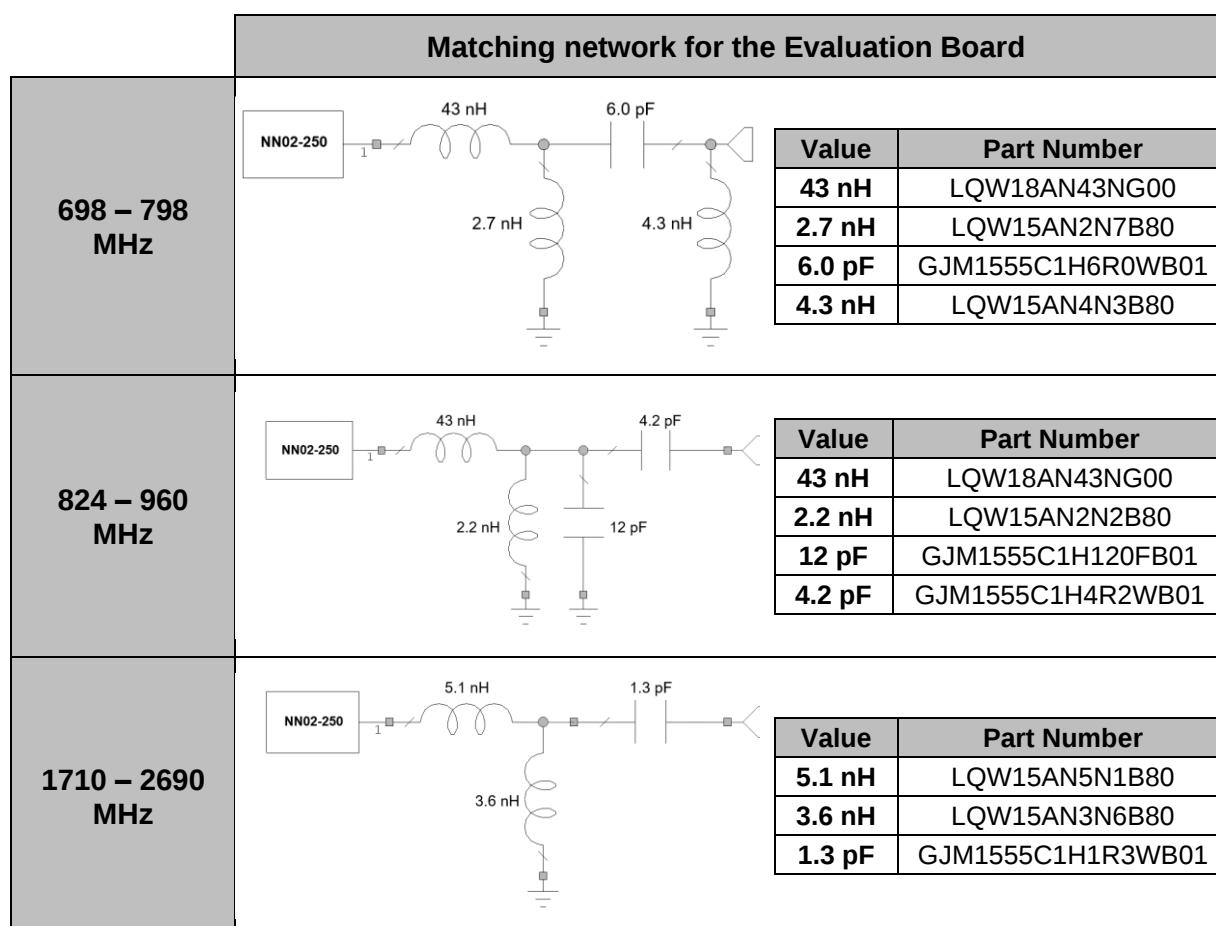
Figure 2 – Matching networks for the 3 ports solution (Evaluation Board with UFL cables).
