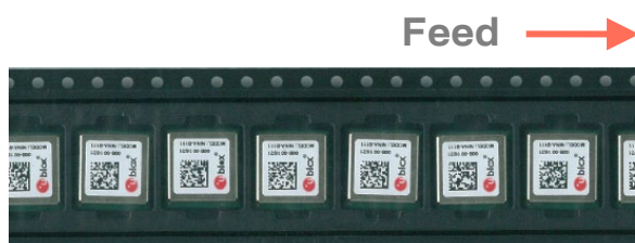
Figure 13: Orientation of NINA-W151 module on tape
