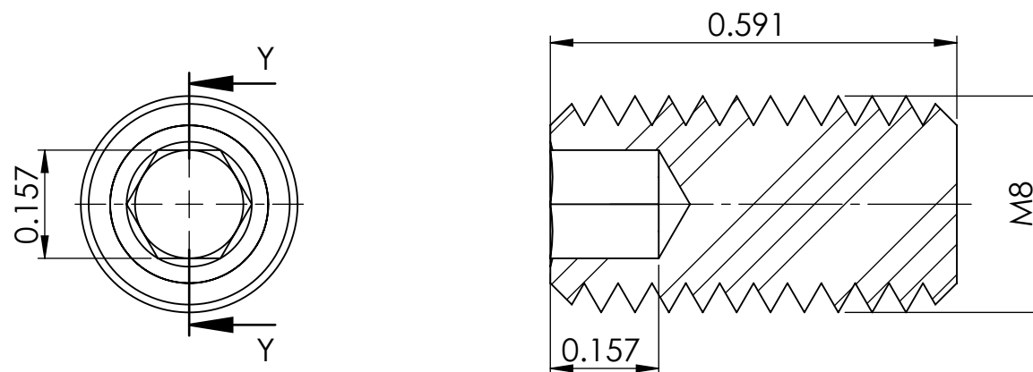
SECTION Y-Y
