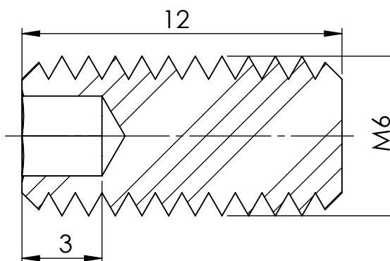
SECTION Y-Y
