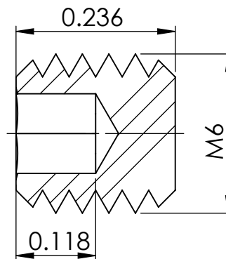
SECTION Y-Y
