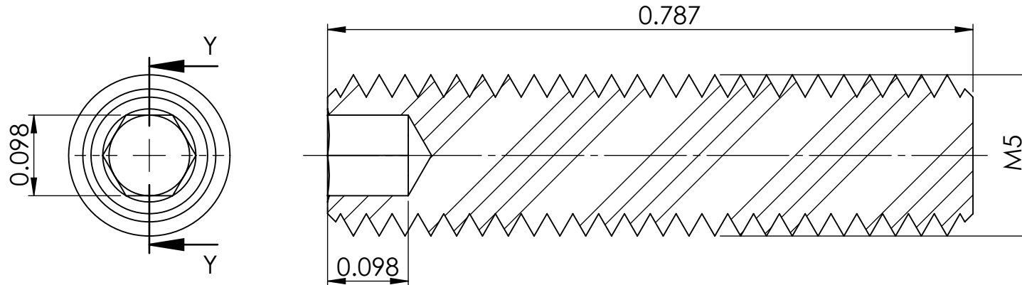
SECTION Y-Y
