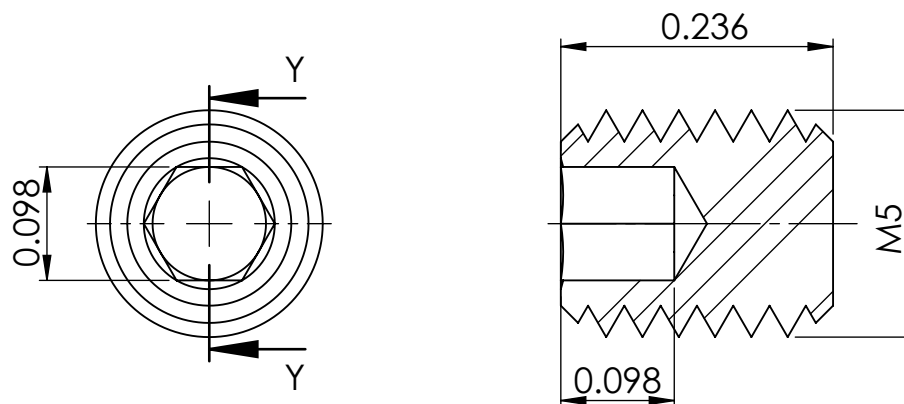
SECTION Y-Y
