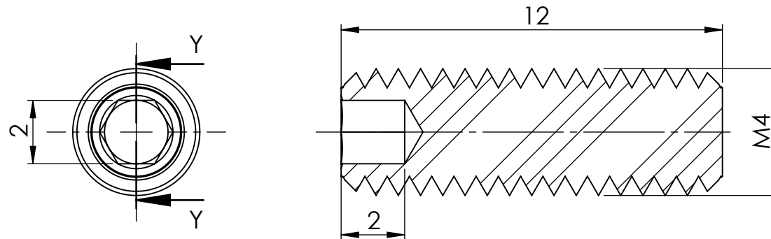
SECTION Y-Y
