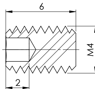
SECTION Y-Y
