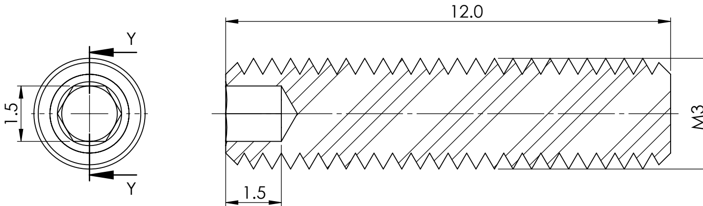
SECTION Y-Y
