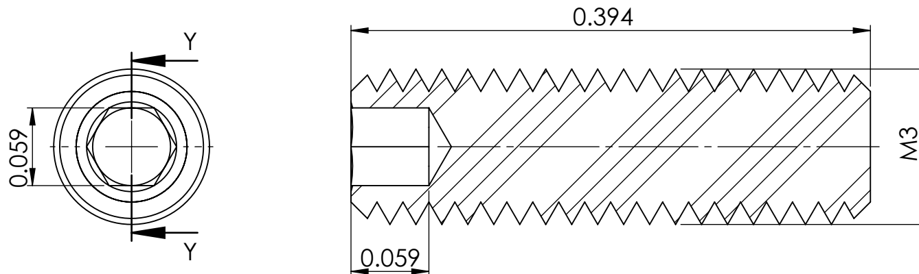
SECTION Y-Y
