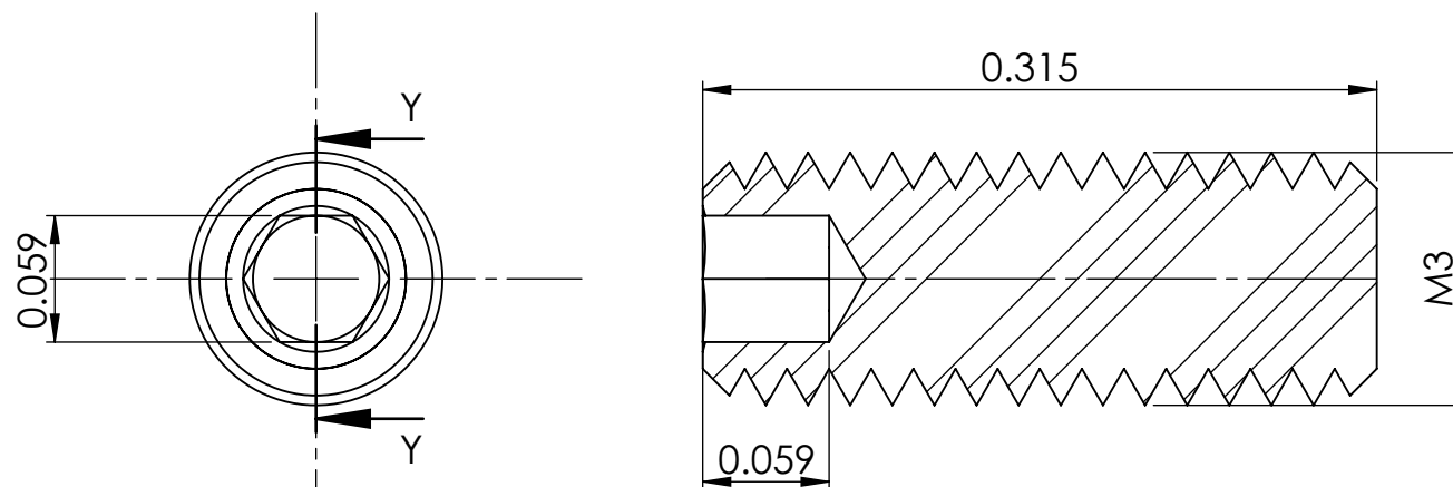
SECTION Y-Y
