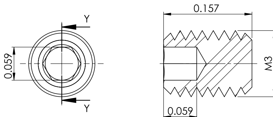
SECTION Y-Y
