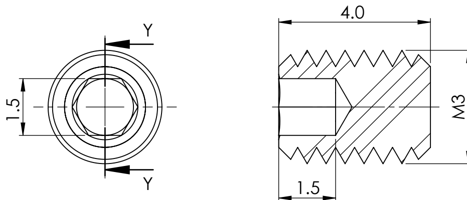
SECTION Y-Y
