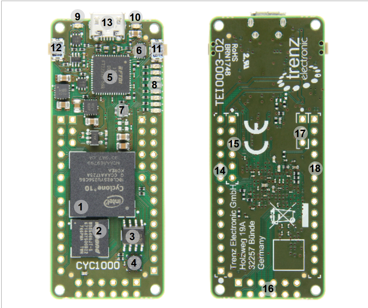
2 Figure 2: TEI0003-02 FPGA module
