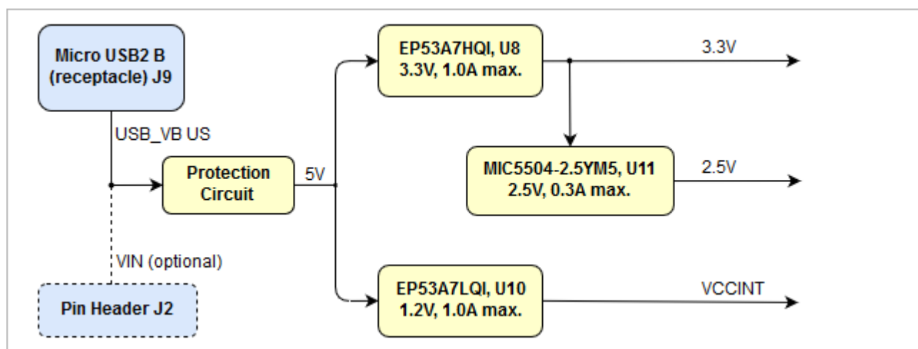
3 Figure 3: Power Distribution Diagram
