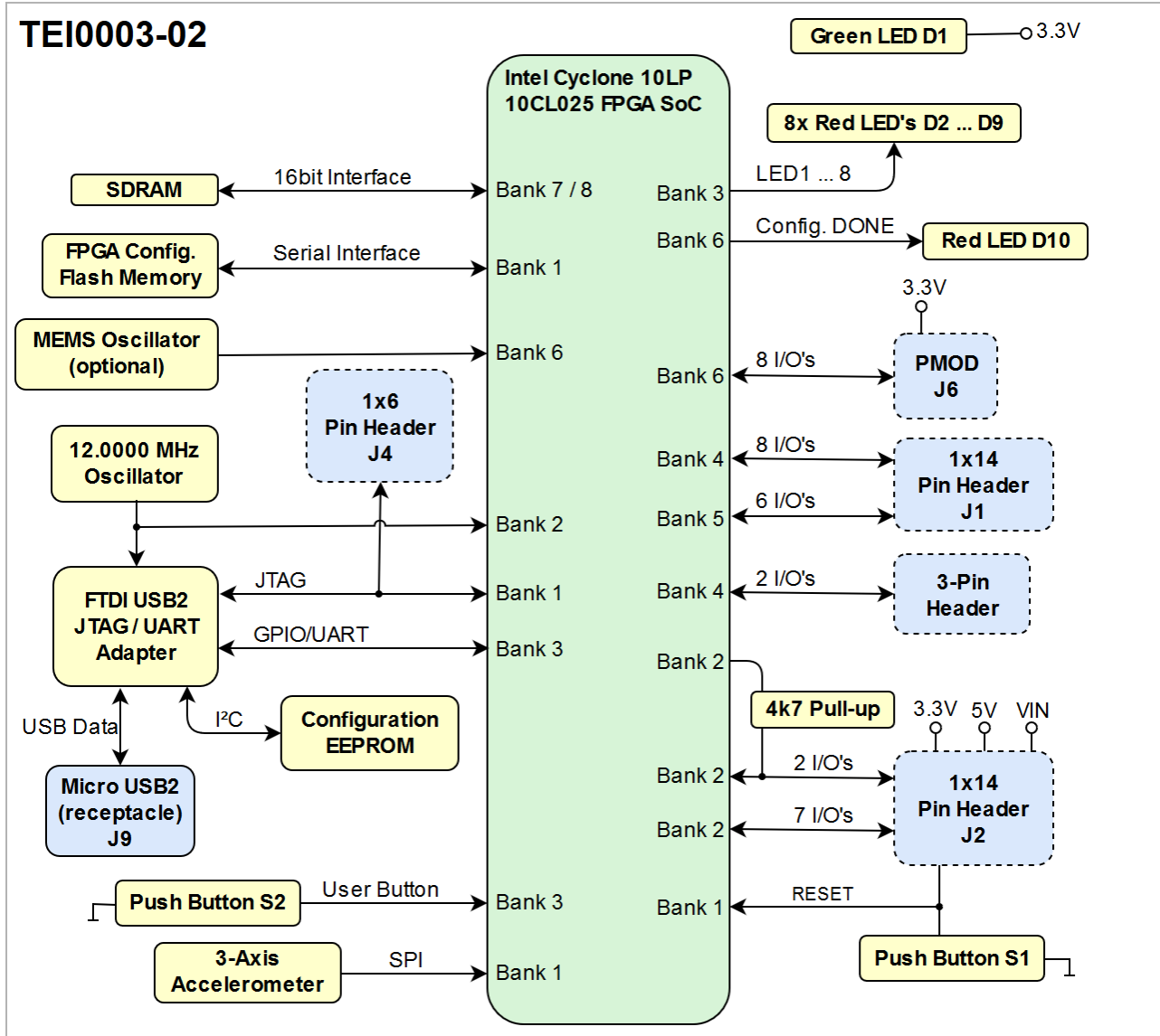
1 Figure 1: TEI0003-02 block diagram
