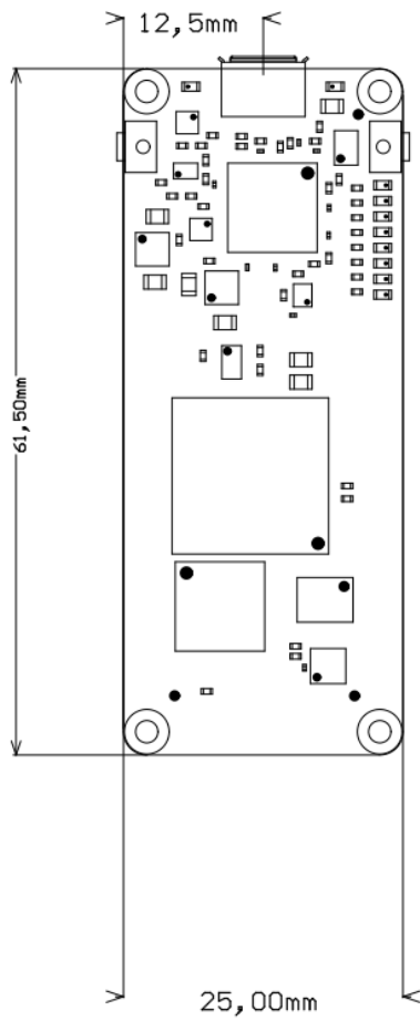
4 Figure 4: Module physical dimensions drawing
