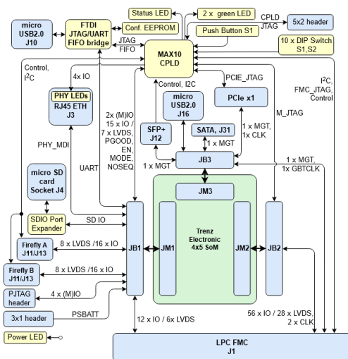
Figure 1: TEF1002 block diagram
