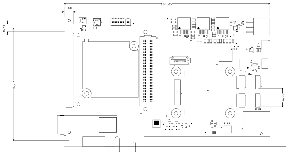
Figure 5: Physical dimensions drawing
