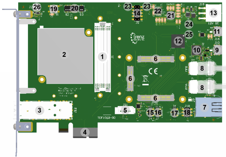
Figure 2: TEF1002 main components
