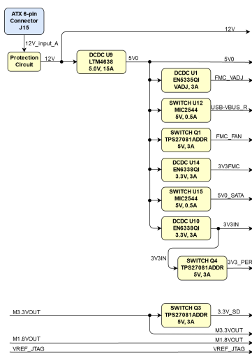
Figure 3: Power Distribution
