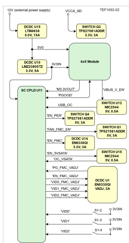
Figure 4: Power Sequence
