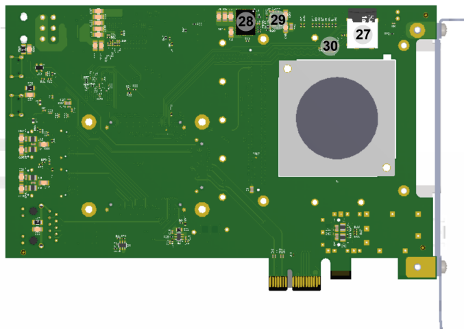
Figure 2: TEF1002 main components
