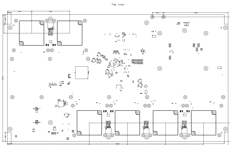
Figure 20: Figure 20: Board physical dimensions drawing
