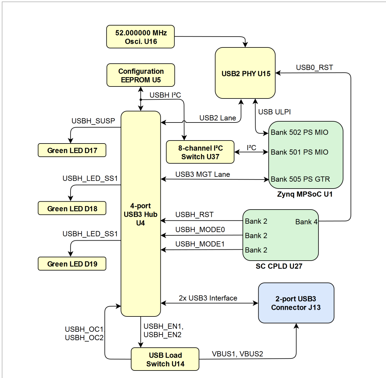
Figure 6: Figure 6: USB3 interface
