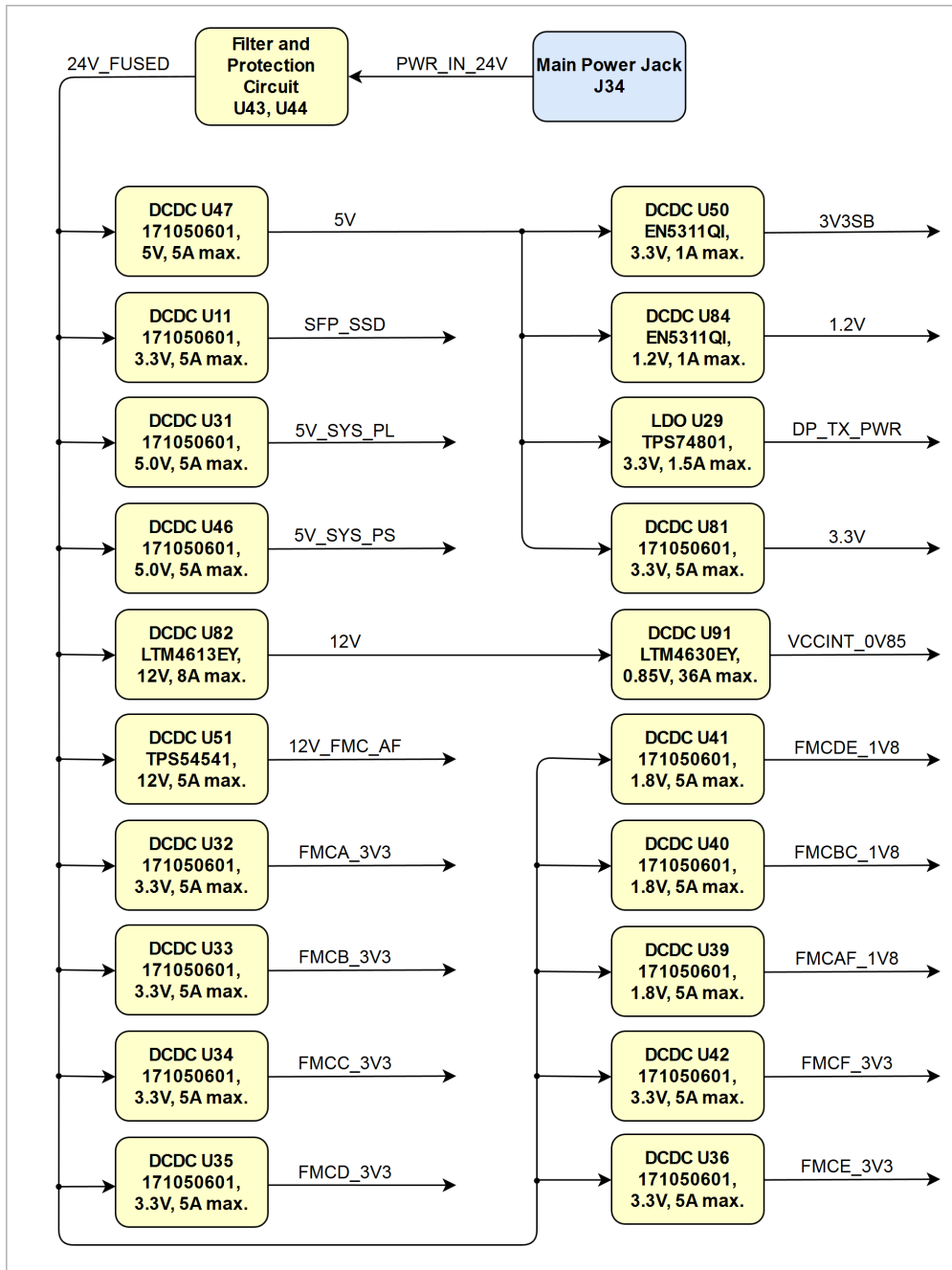
Figure 16: Figure 16: Power distribution diagram
