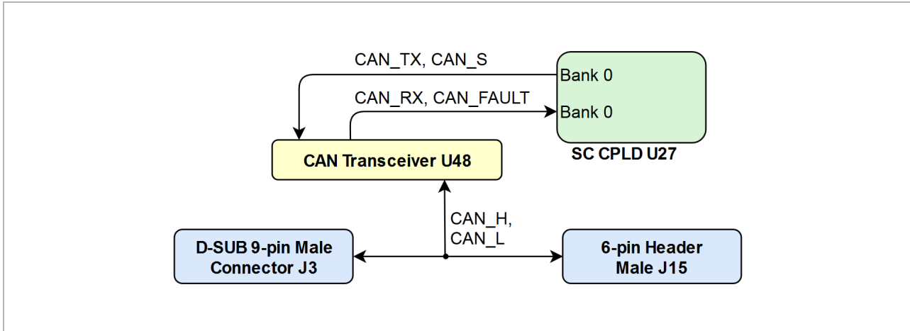
Figure 11: Figure 11: CAN interface
