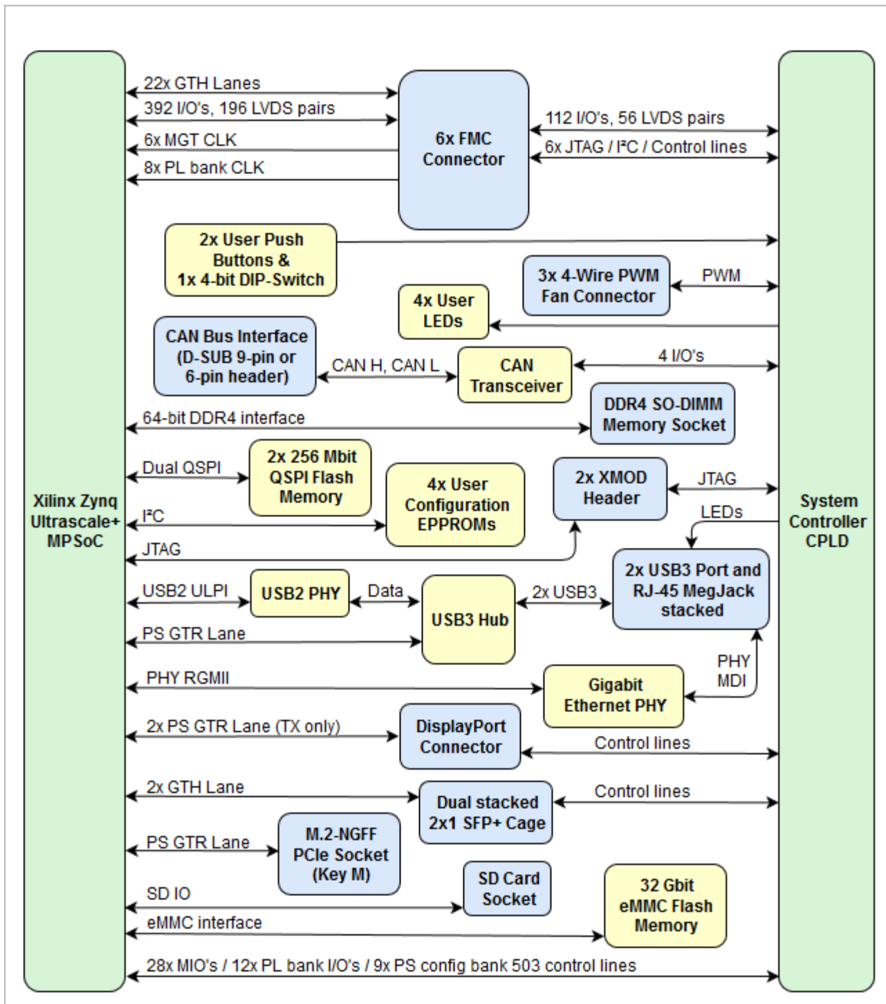
Figure 1: Figure 1: TEB0911-03 block diagram
