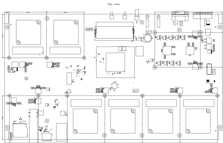
Figure 19: Figure 19: Board physical dimensions drawing
