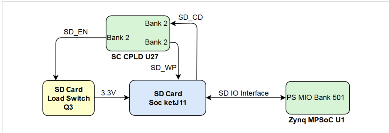
Figure 12: Figure 12: SD Card interface
