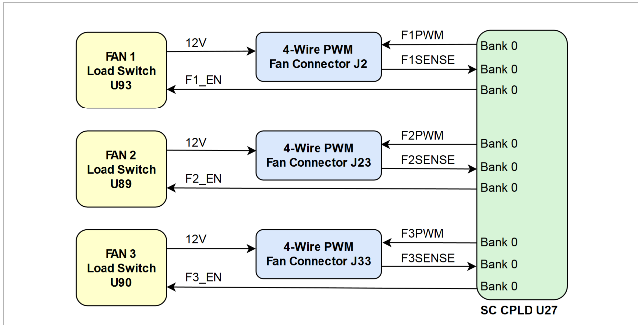
Figure 13: Figure 13: 4-wire PWM FAN connectors
