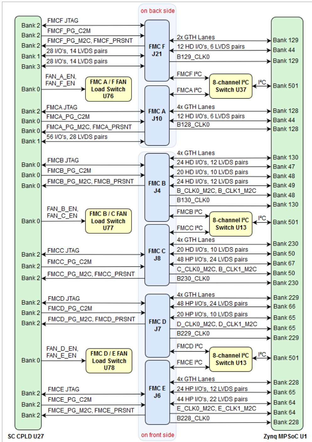
Figure 3: Figure 3: General overview of the FMC connectors
