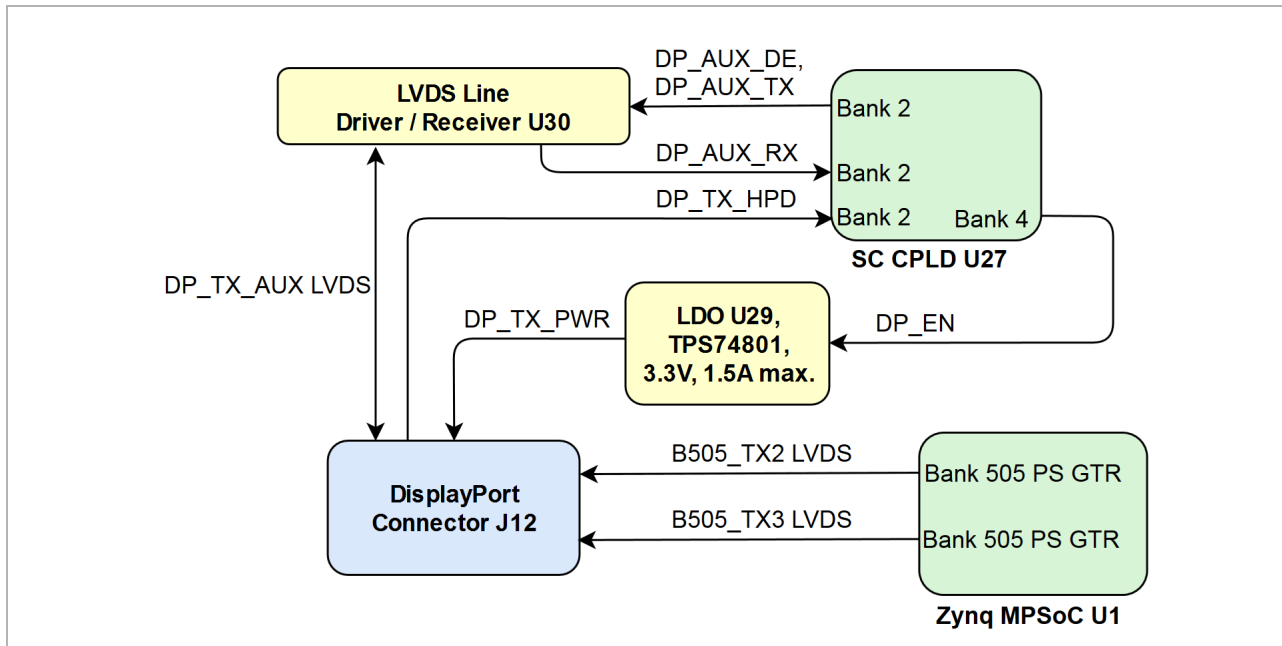
Figure 9: Figure 9: DisplayPort interface
