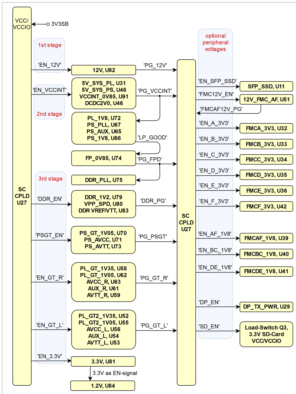
Figure 18: Figure 18: Power-On sequence diagram
