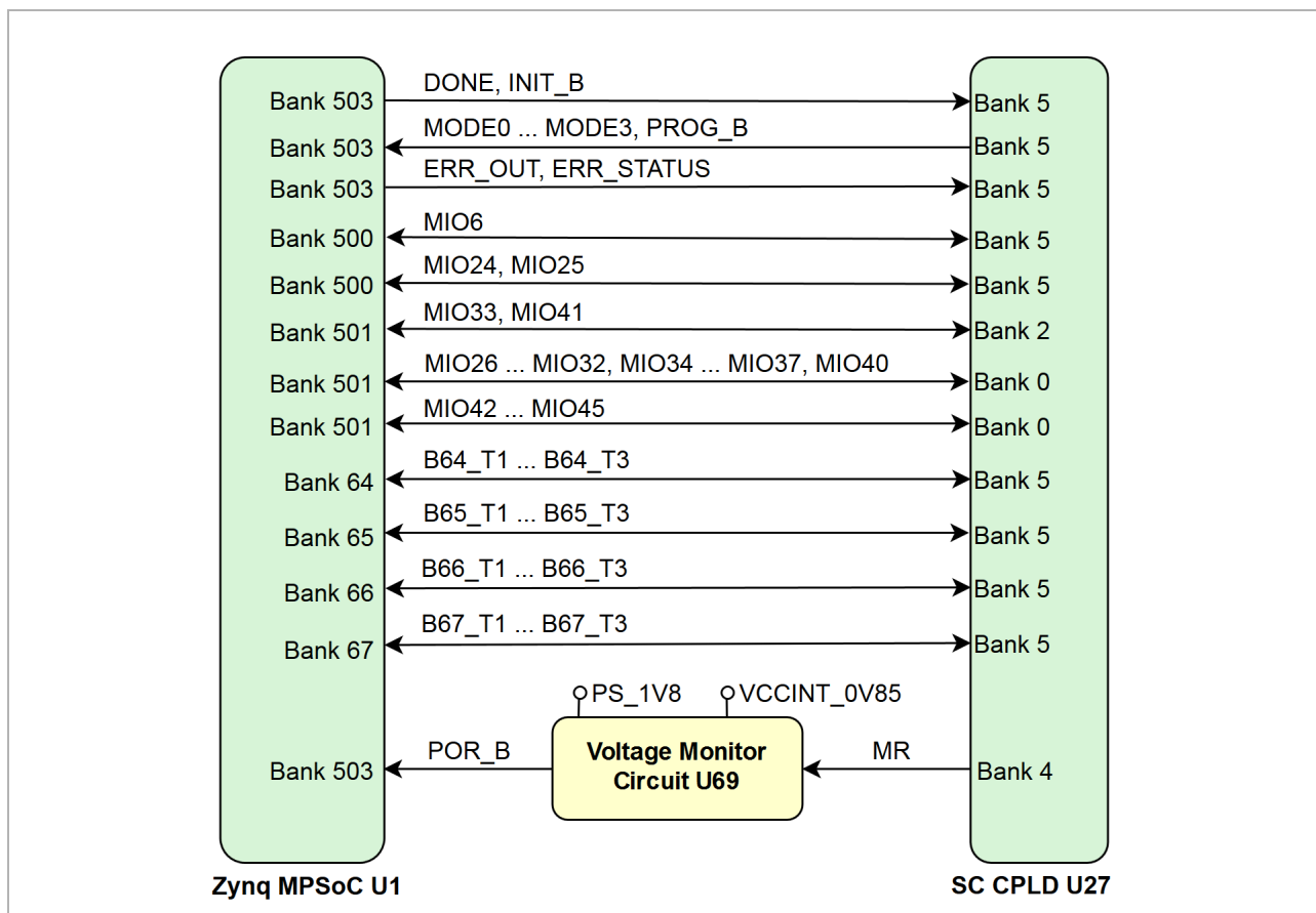
Figure 15: Figure 15: I/O's connecting Zynq MPSoC and SC CPLD
