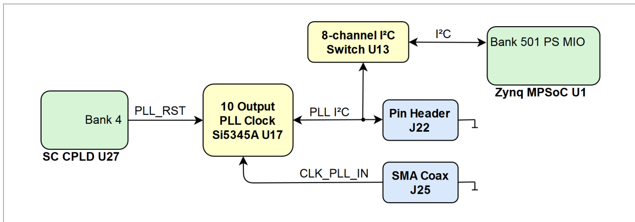
Figure 14: Figure 14: PLL clock interface
