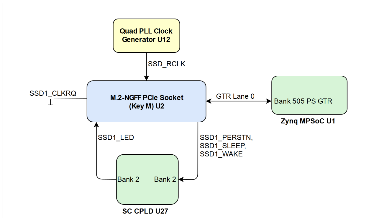
Figure 8: Figure 8: SSD interface
