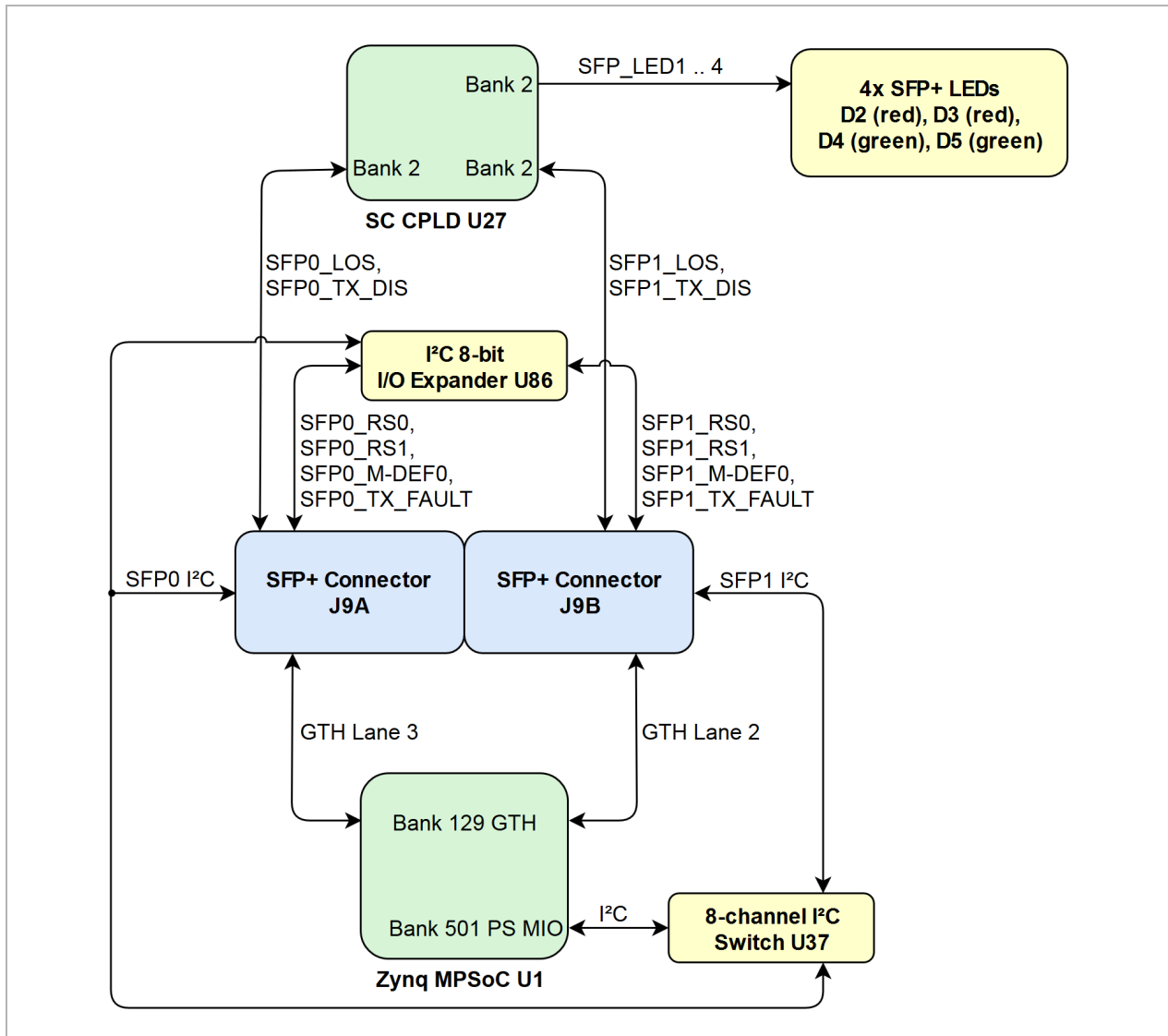
Figure 7: Figure 7: SFP+ interface
