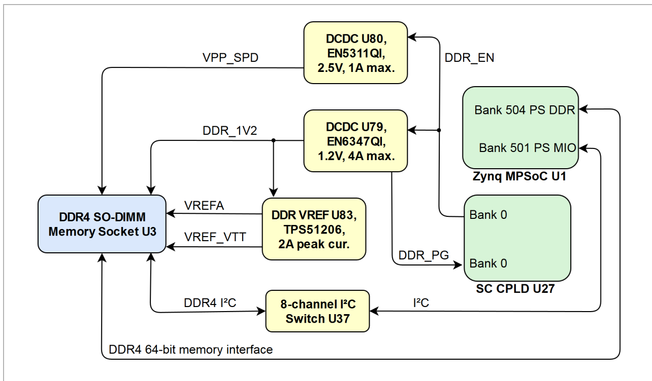
Figure 10: Figure 10: DDR4 memory interface
