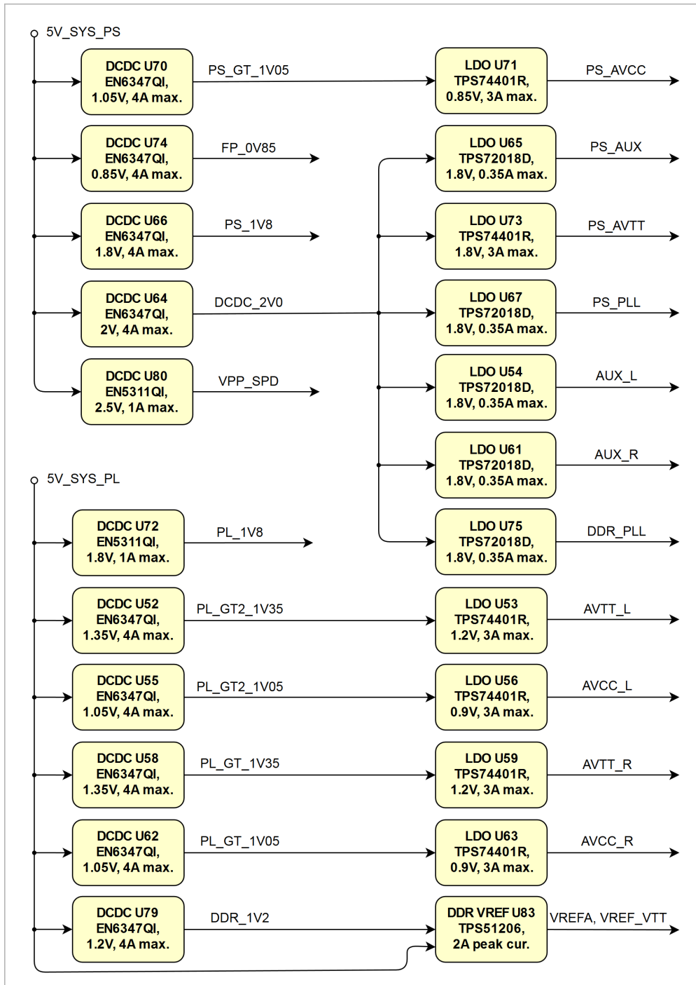
Figure 17: Figure 17: Power distribution diagram continued
