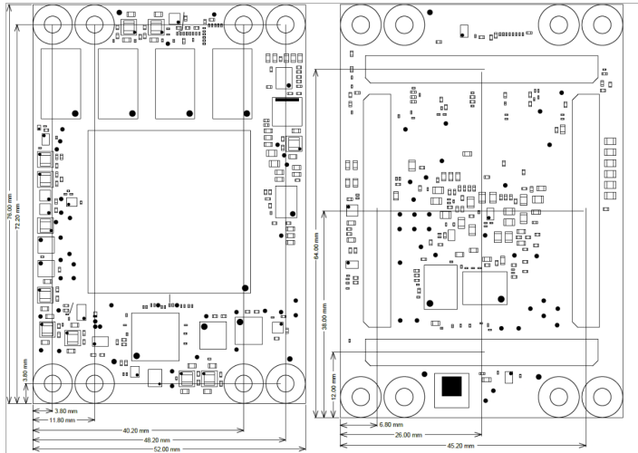
Figure 3: Physical Dimension
