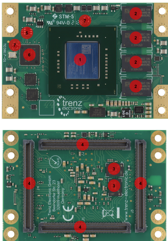
Figure 2: TE0817 main components
