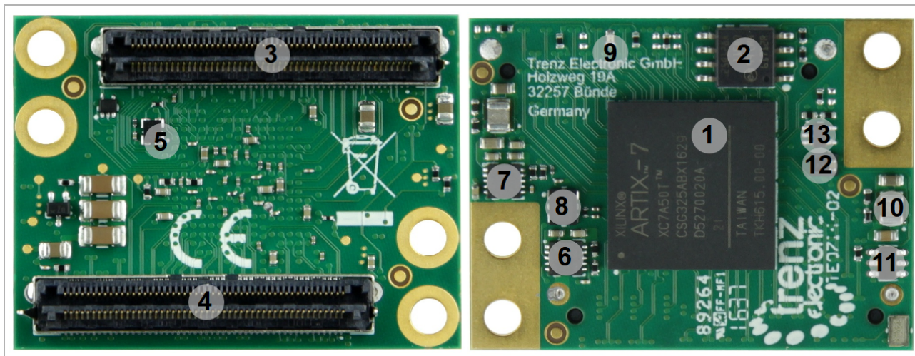
Figure 2: TE0714 main components
