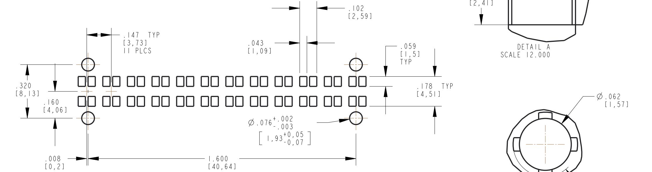
RECOMMENDED SOLDER PAD & HOLES LAYOUT
