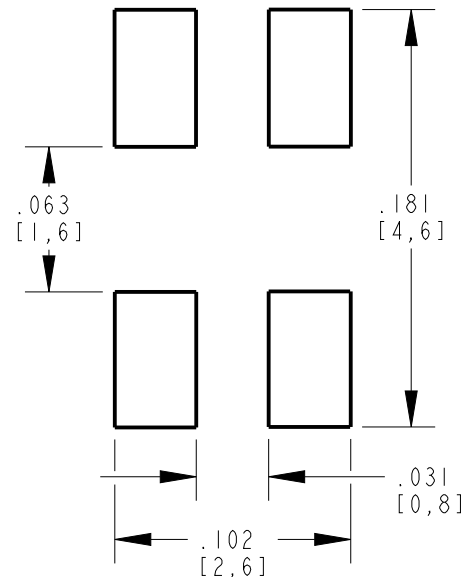
RECOMMENDED SOLDER PAD LAYOUT (TOLERANCE: \pm .004 )
