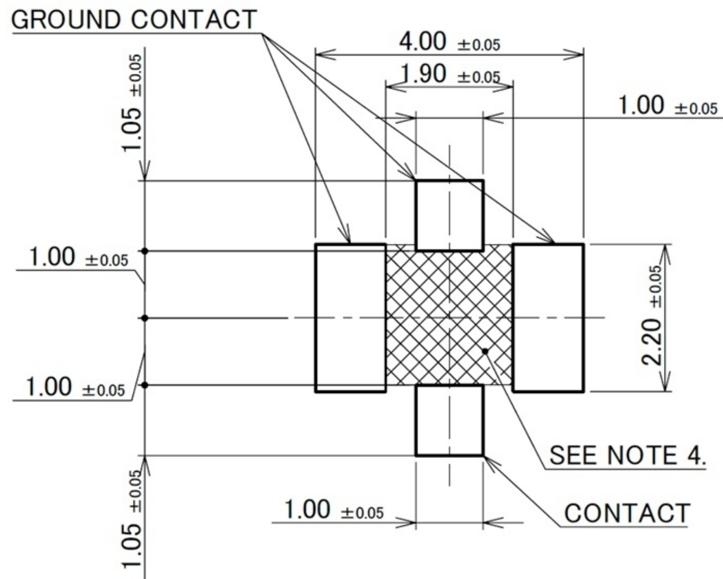
RECOMMENDED FOOTPRINT PATTERN
