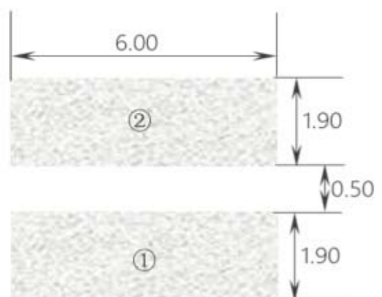
Soldering patterns
