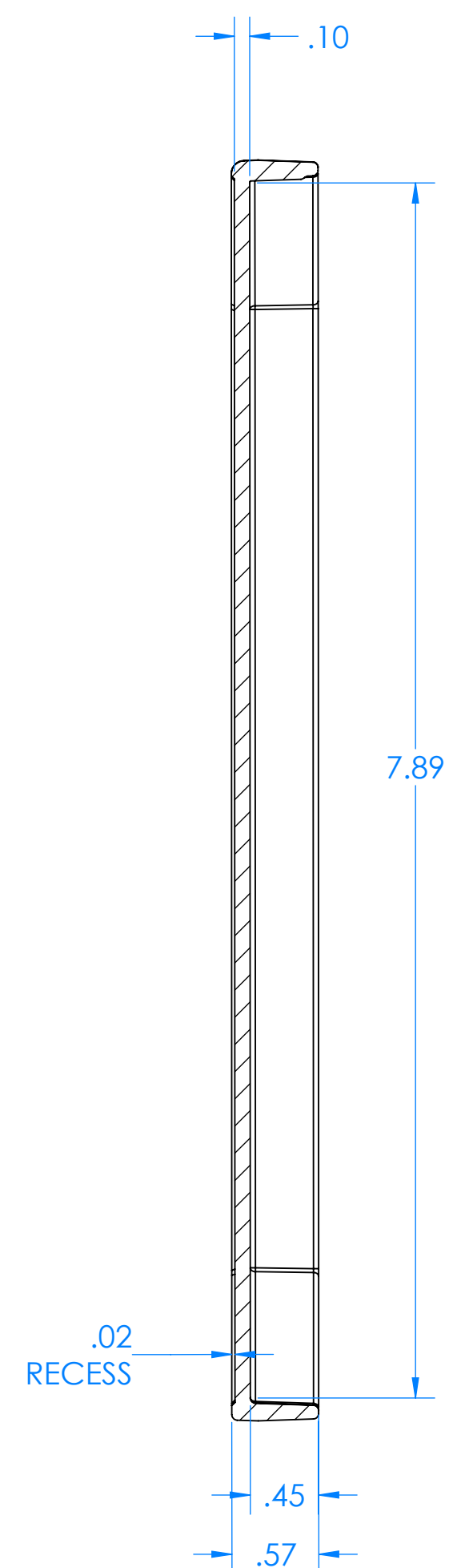
SECTION E-E
