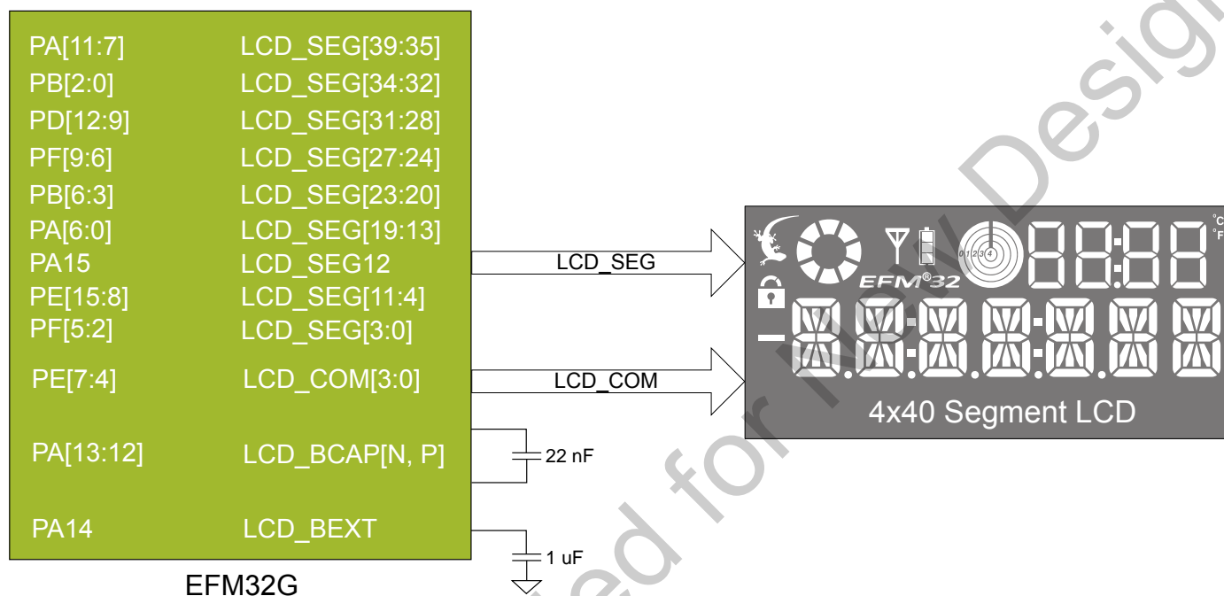
Figure 6.2. Segment LCD
