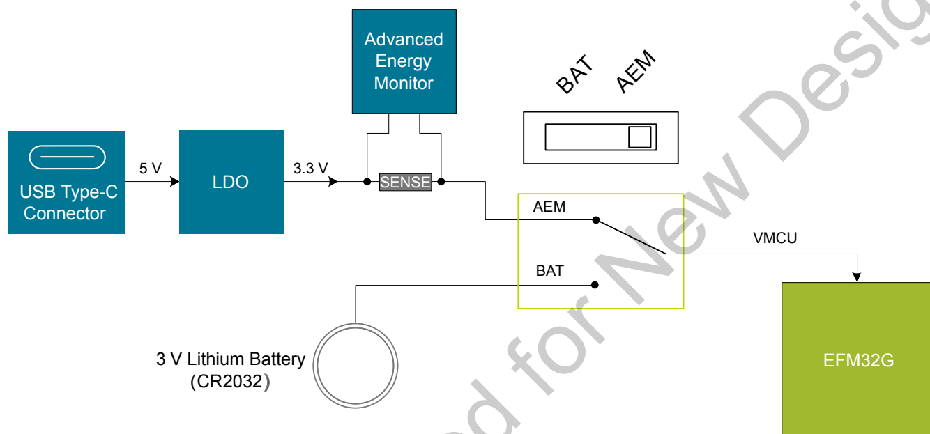
Figure 5.1. Power Switch
