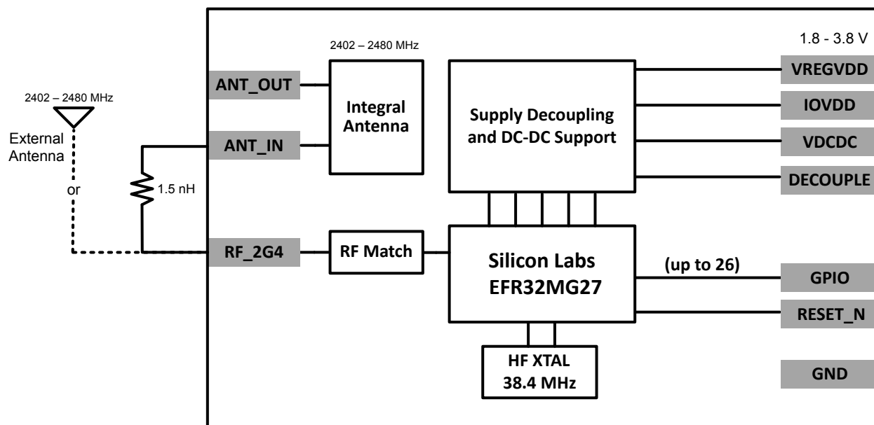
Figure 3.1. MGM270S Block Diagram
