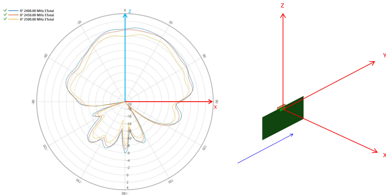
Figure 4.3. MGM270S Typical 2D Antenna Radiation Patterns on 55 mm x 30 mm board - \Phi = 0^\circ Gain (dBi)
