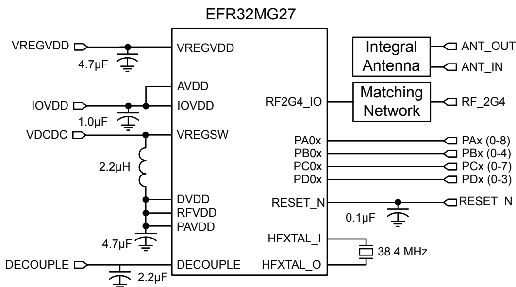
Figure 3.2. MGM270S Module Schematic
