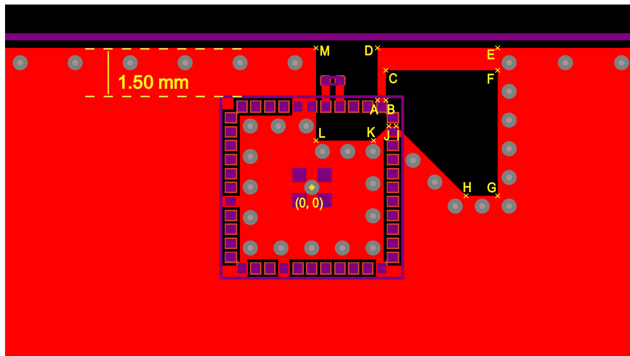
Figure 7.2. TOP Layer Antenna Layout With Coordinates
