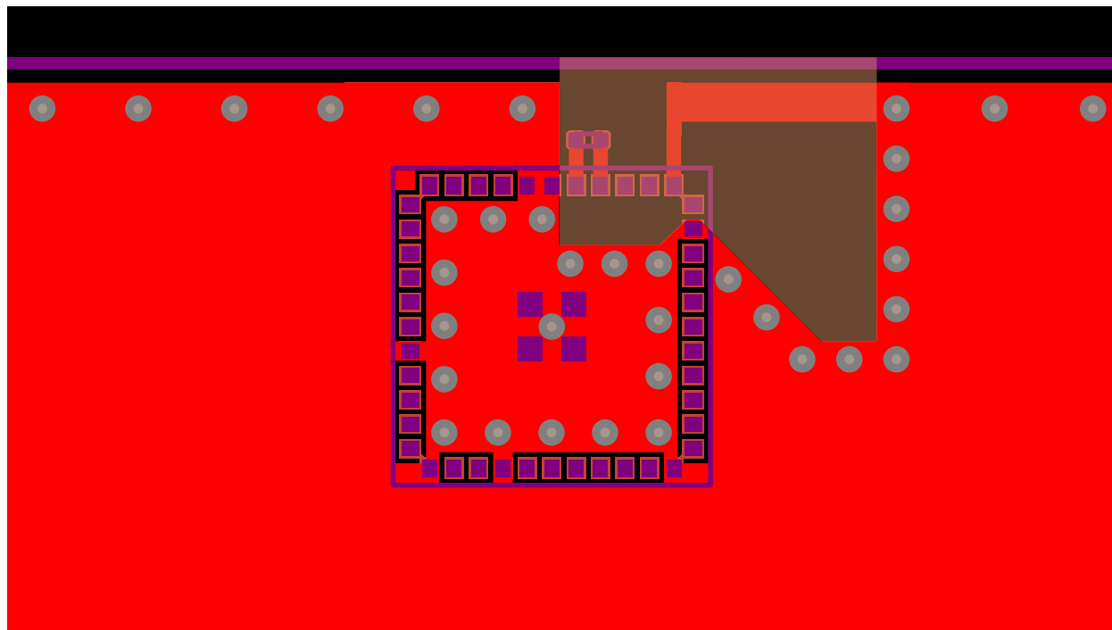
Figure 7.3. Antenna Clearance in Inner and Bottom Layers
