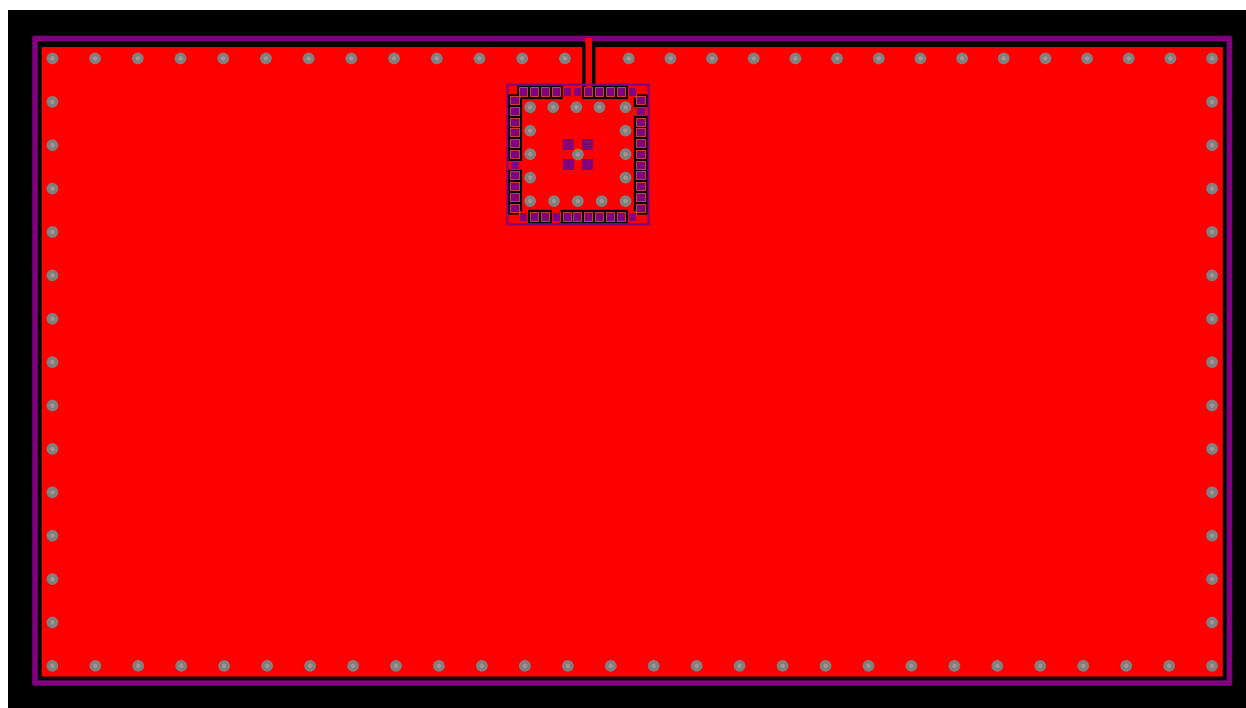
Figure 7.4. Recommended Layout for MGM270S (External Antenna)
