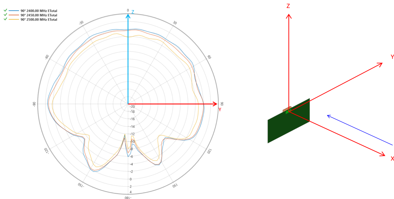
Figure 4.4. MGM270S Typical 2D Antenna Radiation Patterns on 55 mm x 30 mm board - \Phi = 90^\circ Gain (dBi)
