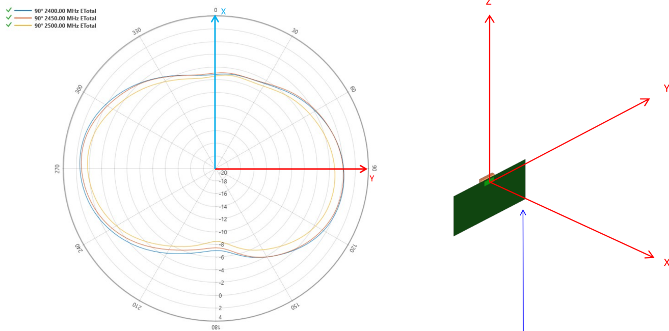
Figure 4.5. MGM270S Typical 2D Antenna Radiation Patterns on 55 mm x 30 mm board - Theta 90° Gain (dBi)
