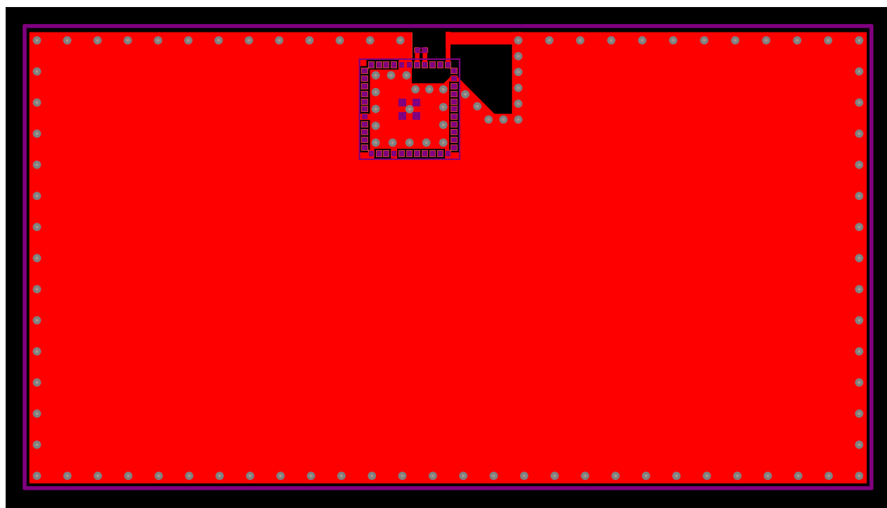
Figure 7.1. Recommended Layout for MGM270S (Integral Antenna)
