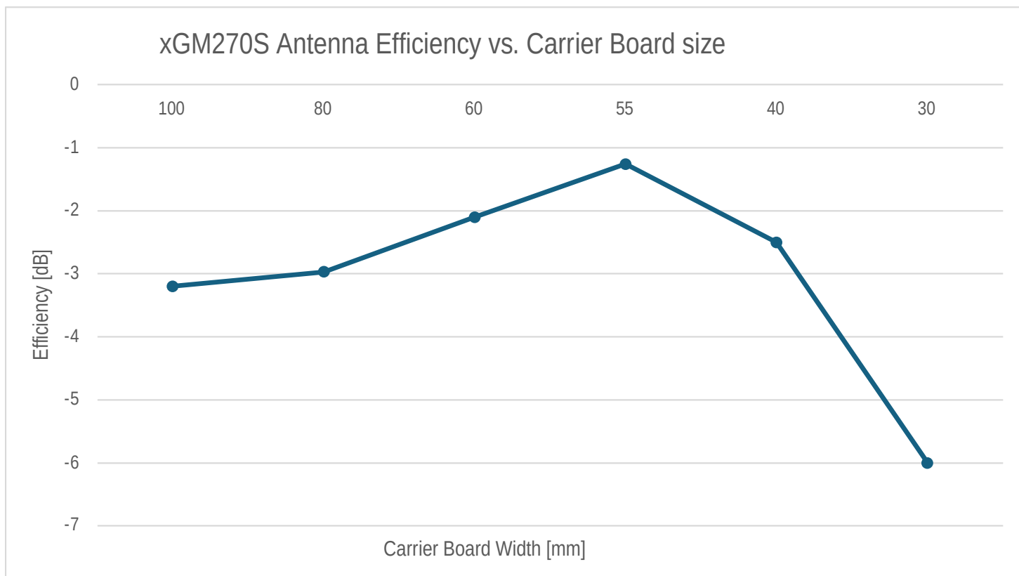
Figure 7.7. Efficiency of the Integrated Antenna as Function of the Carrier Board Size for MGM270S
