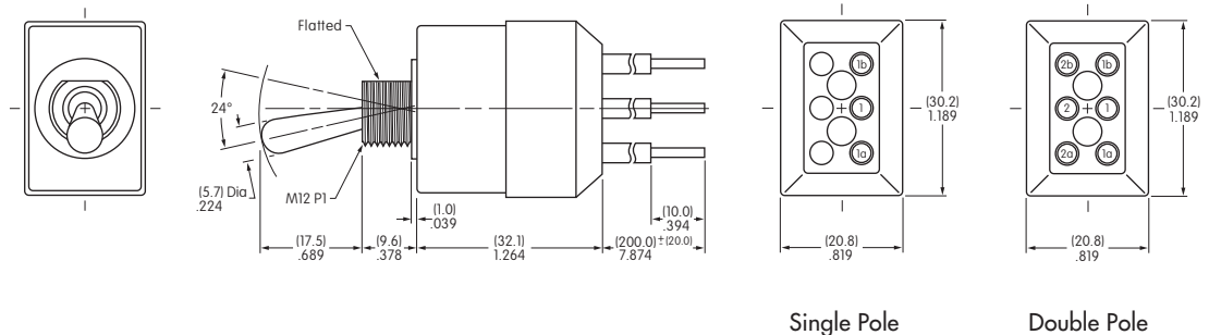
Single Pole
